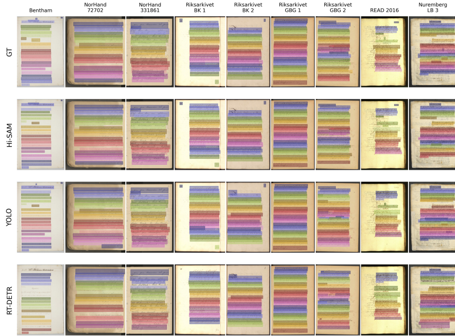
Fig. S-2. Qualitative comparison after pre-training on the Mix dataset and fine-tuning on 10 target dataset page images. The first row shows ground-truth boundary boxes; the remaining rows show the corresponding predictions from each line detection model on a samples from datasets we used in the study.
