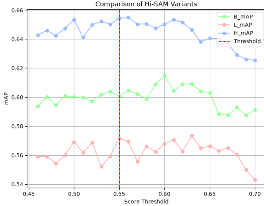
Fig. S-1. Segmentation performance of the Hi-SAM Base (B), Large (L), and Huge (H) variants at different confidence score thresholds, measured using mAP_{50:95} .
